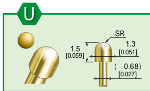
K2-1.0Ⅲ U-4.5M1.3-3 Plunger Material: BeCu
