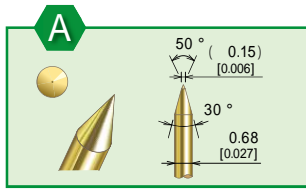
K2-1.0Ⅲ A-4.5M-6 Plunger Material: SK (Steel)
