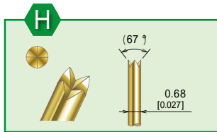
K2-1.0Ⅲ H-4.5M-3 Plunger Material: SK (Steel)
