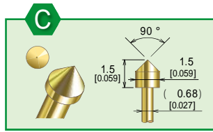
K2-1.0Ⅲ C-4.5M1.5-5 Plunger Material: BeCu
