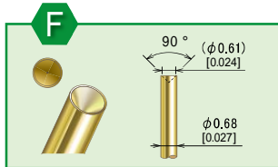
K2-1.0Ⅲ F-4.5M-4 Plunger Material: BeCu
