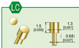
K2-1.0Ⅲ LC-4.5M1.3-3 Plunger Material: SK (Steel)
