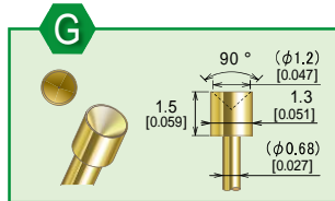
K2-1.0Ⅲ G-4.5M1.3-3 Plunger Material: BeCu
