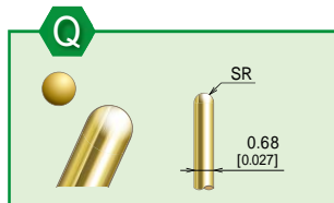
K2-1.0Ⅲ Q-4.5M-4 Plunger Material: SK (Steel)
