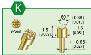
K2-1.0Ⅲ K-4.5M1.3-3 Plunger Material: SK (Steel)
